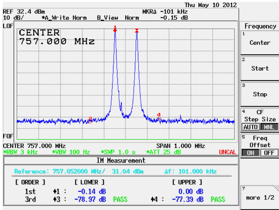
< IMD @ 757MHz >
